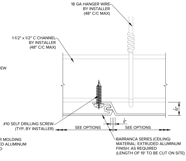
DETAIL B TYP. JOINT CONDITION
