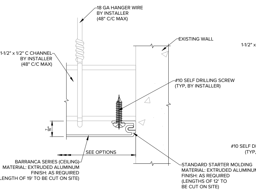
DETAIL A STARTING CONDITION
