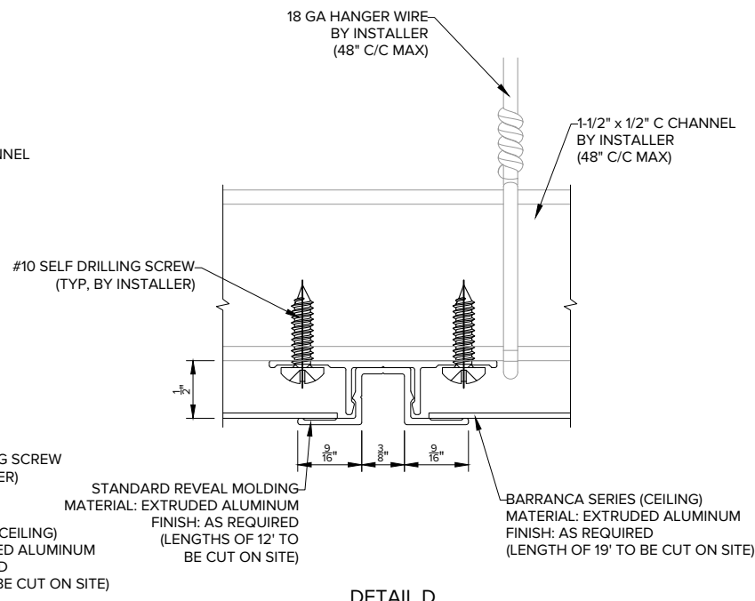
DETAIL D REVEAL COVER
