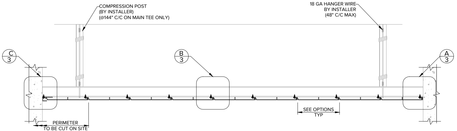
TRANSVERSAL SECTION
