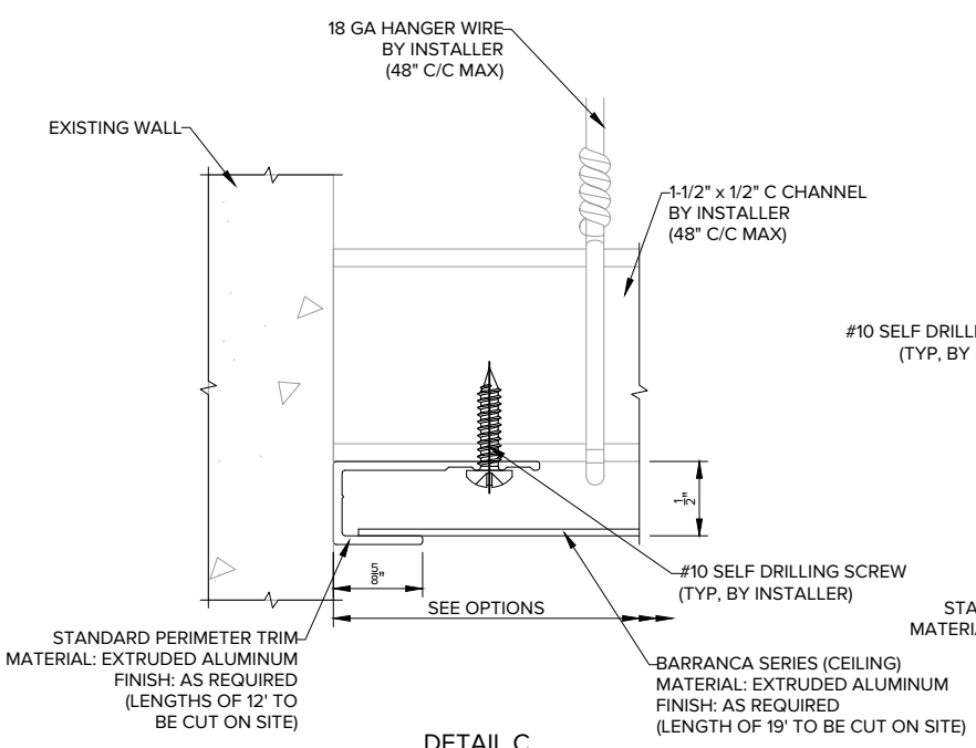
DETAIL C WALL TO WALL CONDITION
