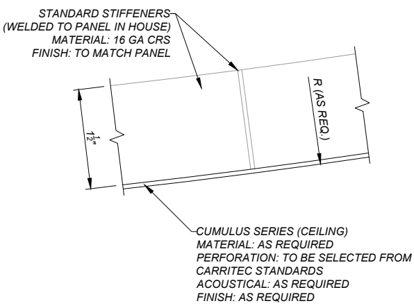
DETAIL B STIFFENER DETAIL
