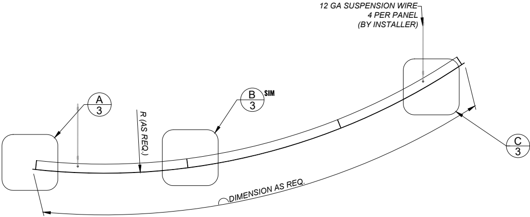
TRANSVERSAL SECTION
