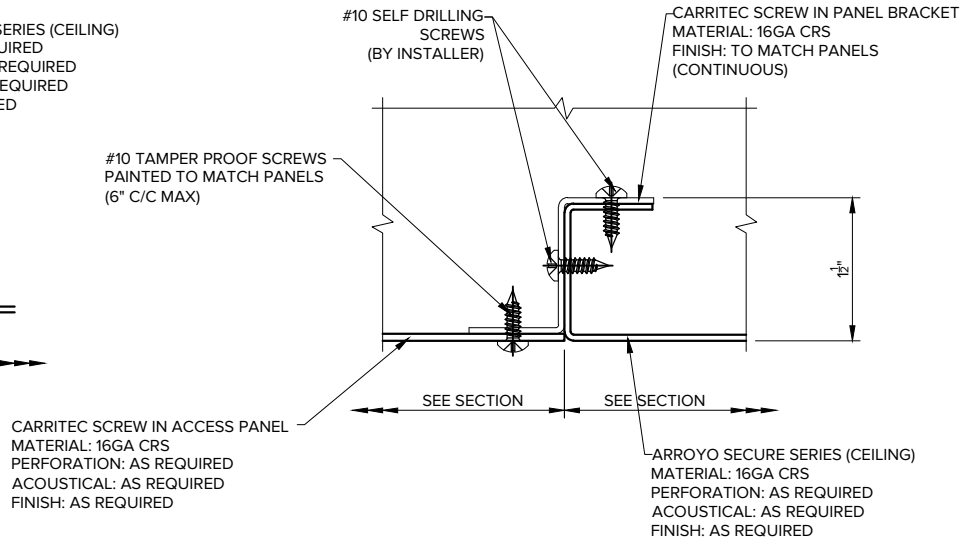
DETAIL D ACCESS PANEL
