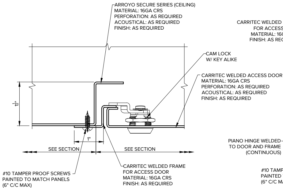
DETAIL E ACCESS DOOR (LOCK)
