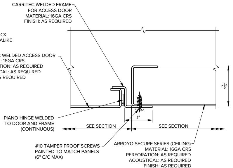
DETAIL F ACCESS DOOR (HINGE)
